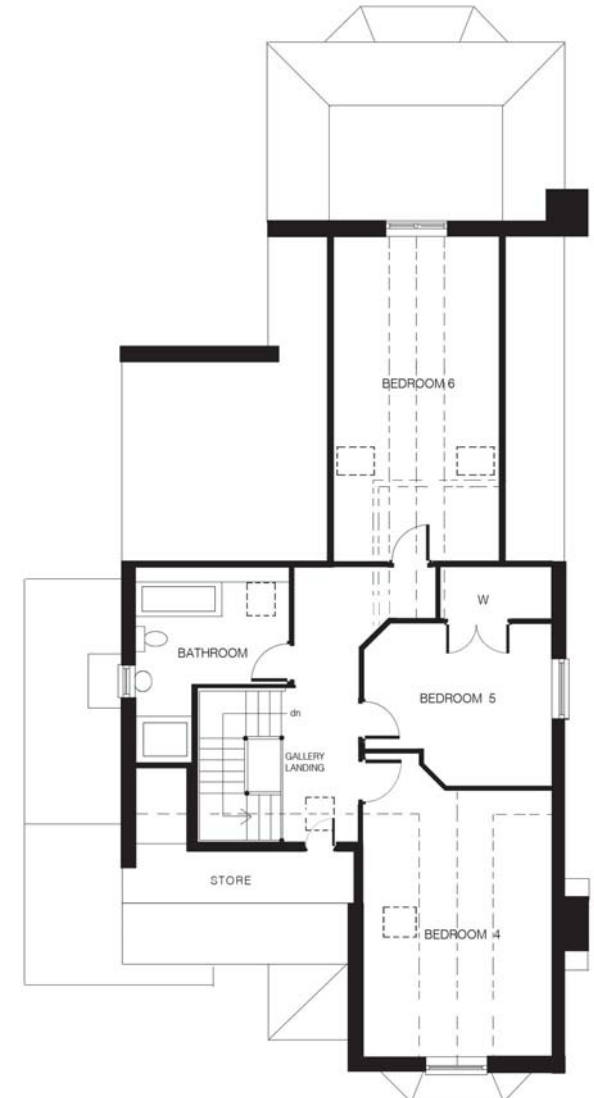
PLOT 1 - SECOND FLOOR
