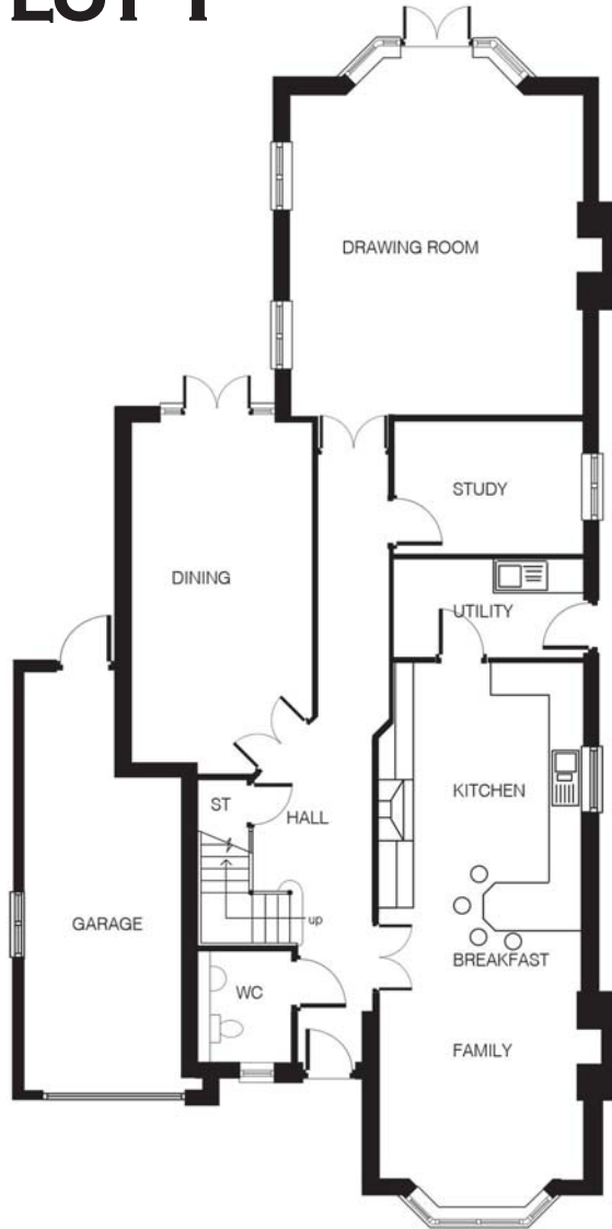
PLOT 1 - GROUND FLOOR
